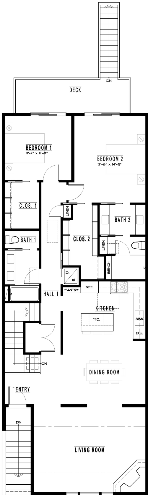
2 MAIN FLOOR PLAN
